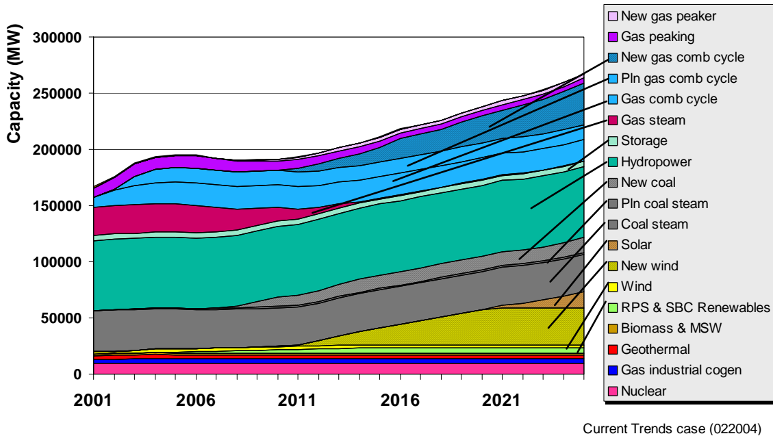
Figure 2-11: Base Case Forecast WECC Resource Mix
