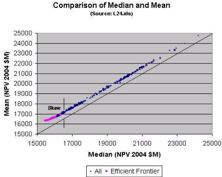
Figure 6-10: Mean vs Median
