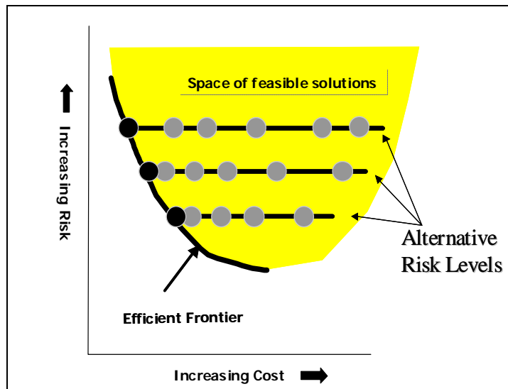
Figure 6-8: Feasibility Space
