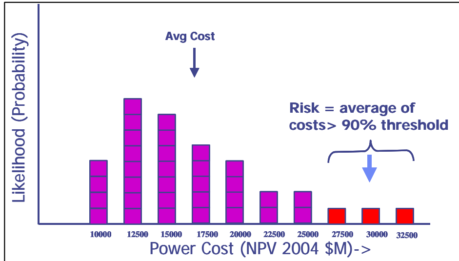
Figure 6-5: TailVaR 90
