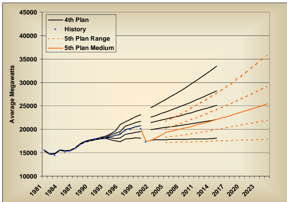
Figure 2-3: Demand Forecast Range Compared to History and Council’s Fourth Power Plan
