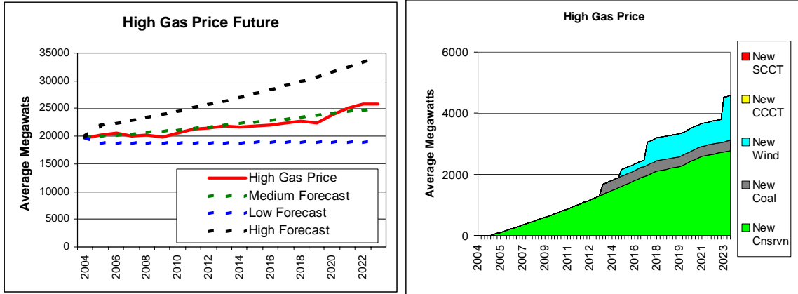
Figure 7-21 Demand Growth and Resource Build Out for a High Gas Price Future
