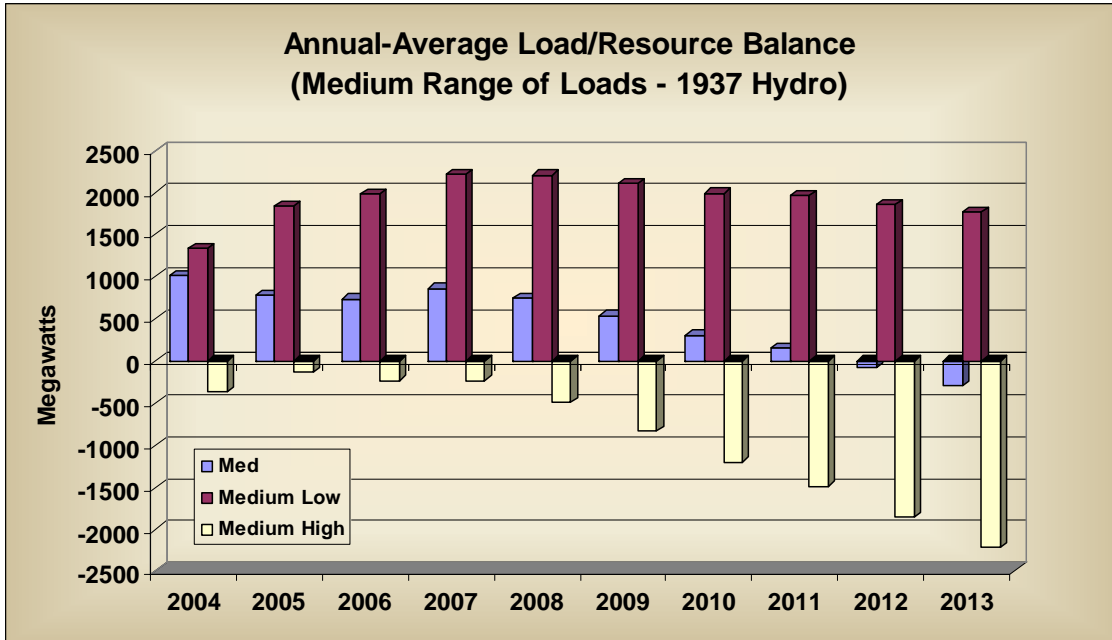
Figure 2-6: Load Resource Balance with Existing Resources Under Medium-Low, Medium And Medium-High Demand Forecasts
