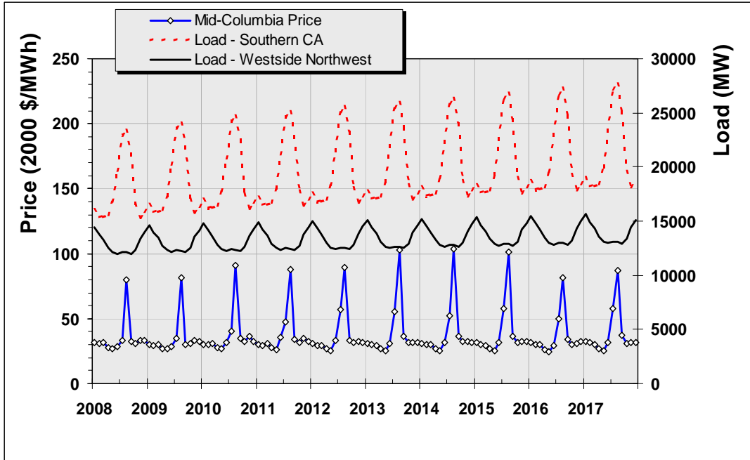
Figure 2-10: Forecast Monthly Wholesale Mid-Columbia Electricity Prices Compared to Northwest and Southwest Loads
