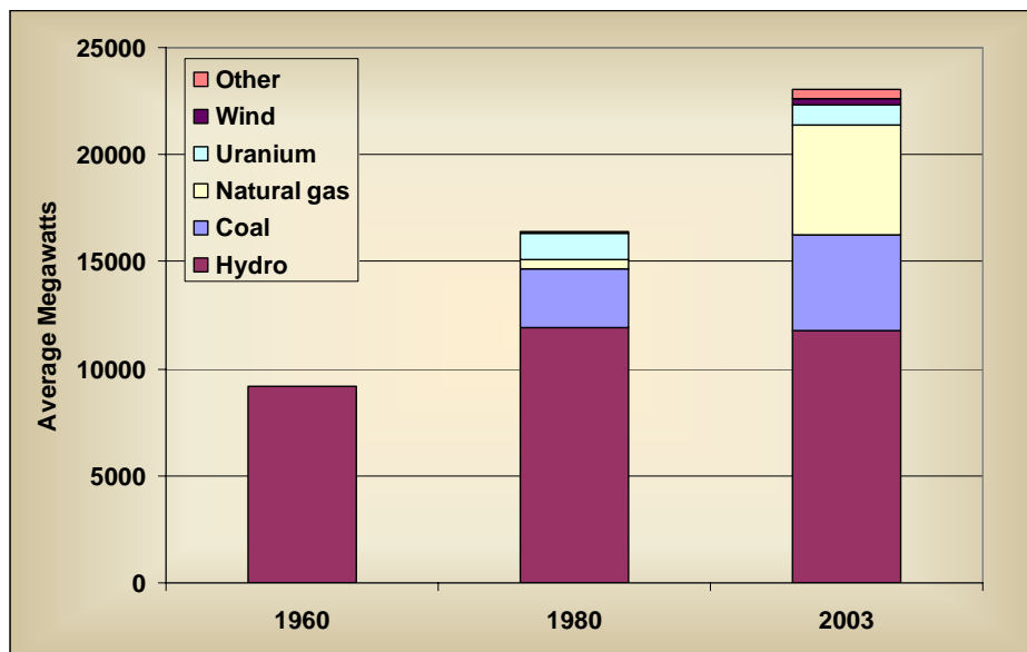
Figure 2-5: Changing Pacific Northwest Sources Electricity Generation
