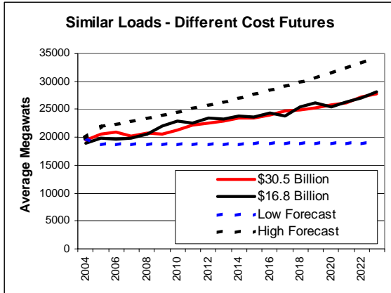
Figure 7-20 Demand Growth for Two Similar Cases with Different Costs
