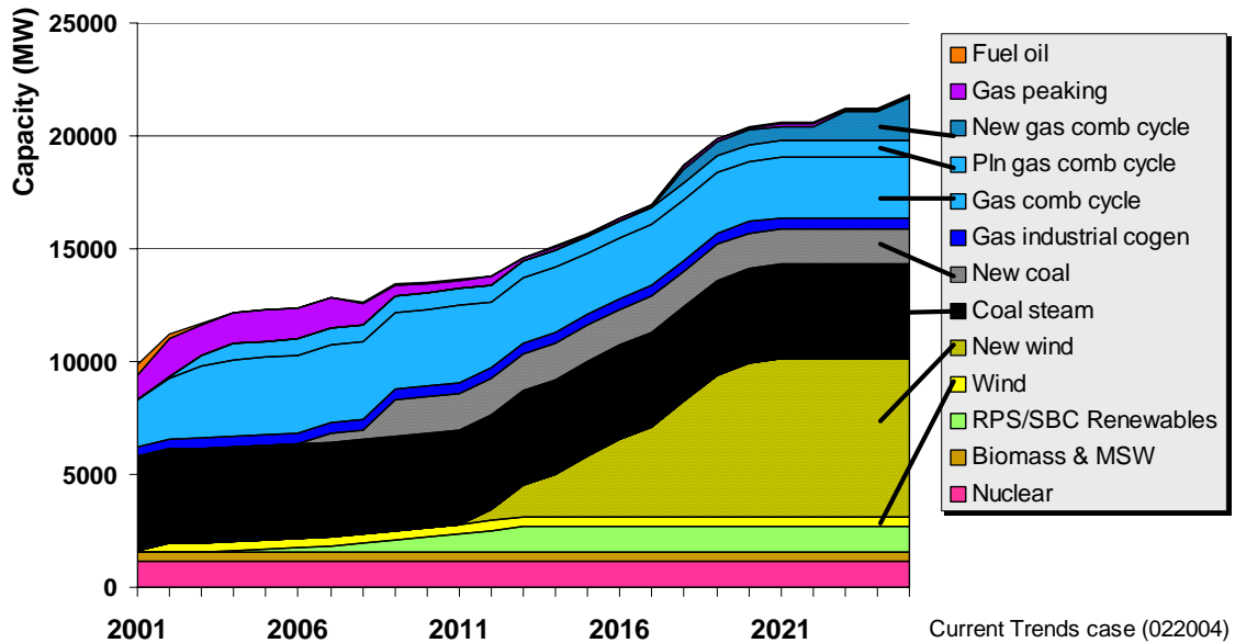
Figure 2-12: Base Case Forecast of Pacific Northwest Resource Mix (Hydro Omitted)
