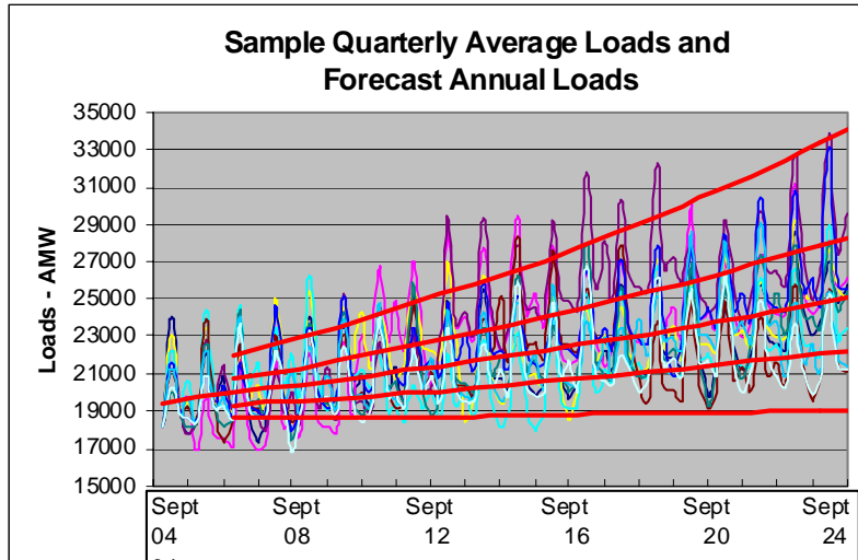
Figure 6-3: Load Futures
