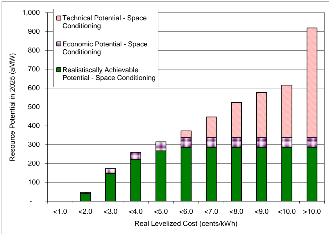
Figure 3-9: Residential Space Conditioning Conservation Resource Potential
