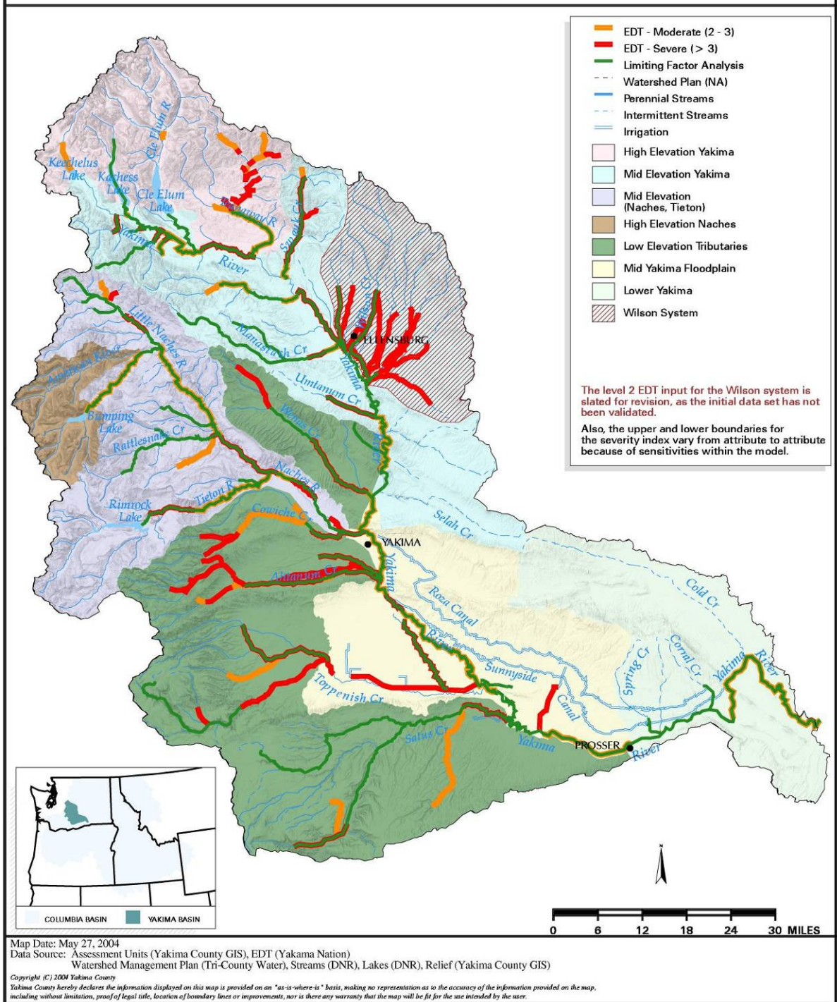
Figure 2-72. EDT and Limiting Factors for hydroconfinement
