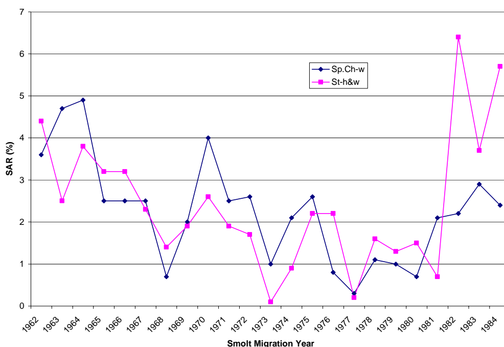
Figure 43 Survival from smolt to returning adult for upper Columbia wild spring Chinook and steelhead stocks as estimated by Raymond (1988). The reference point for smolt abundance is the upper dam on the Columbia and estimated return of adults to that location. Years refer to smolt migration years.
