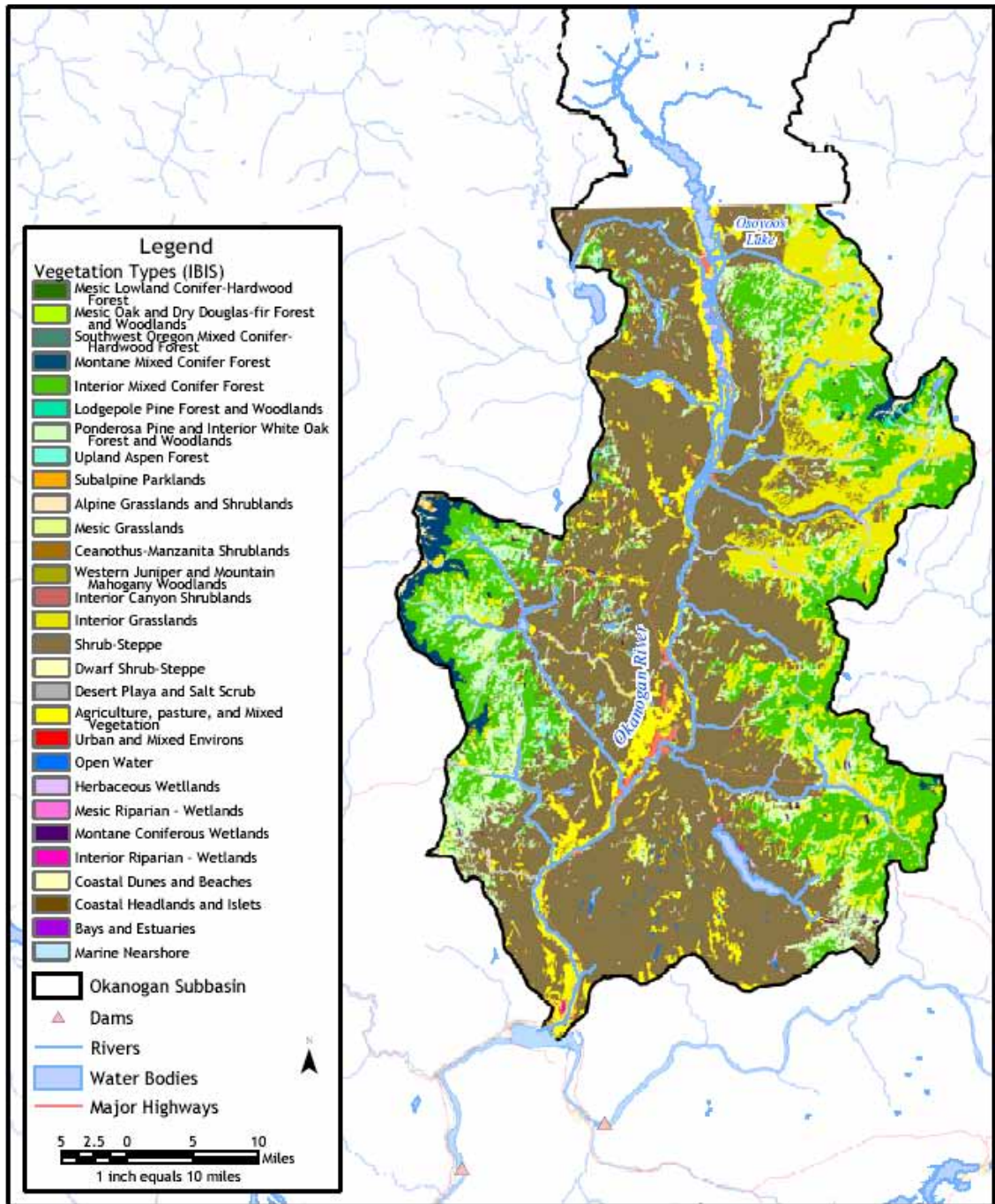
Figure 13. Vegetation Types in the Okanogan subbasin
