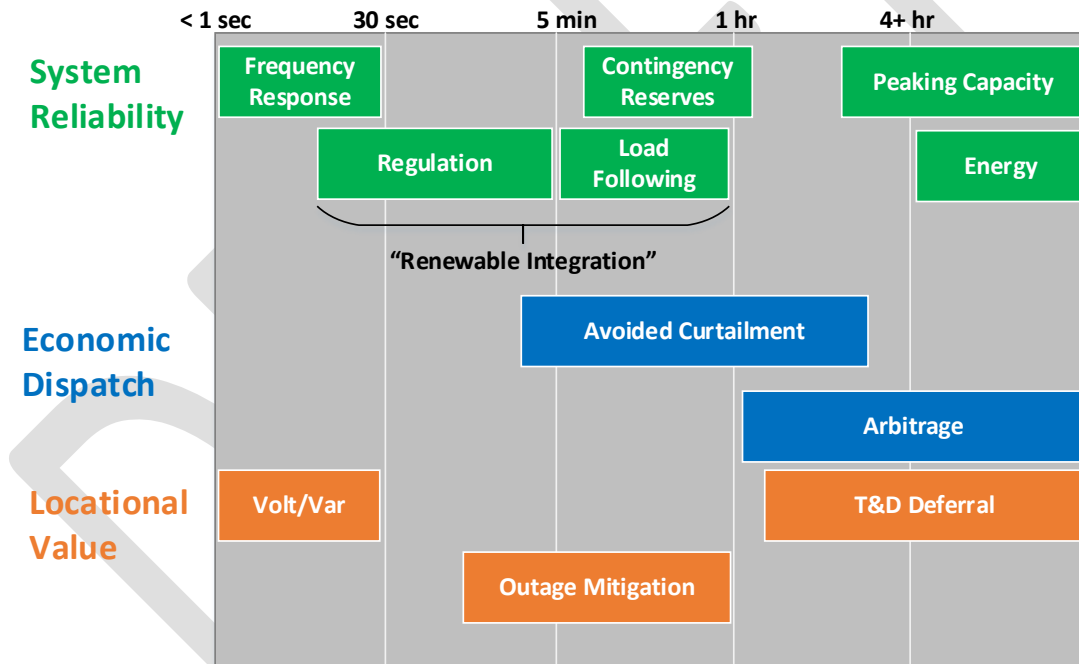
Figure 1: Key value streams within the power system and their associated timescales of action.
